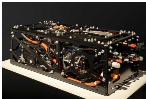
TFCM2-F_3-4 close right angle - Toyota
